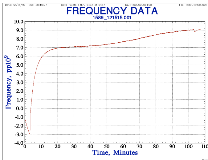
Figure 2 – 9635QT Frequency vs. Total Dose
